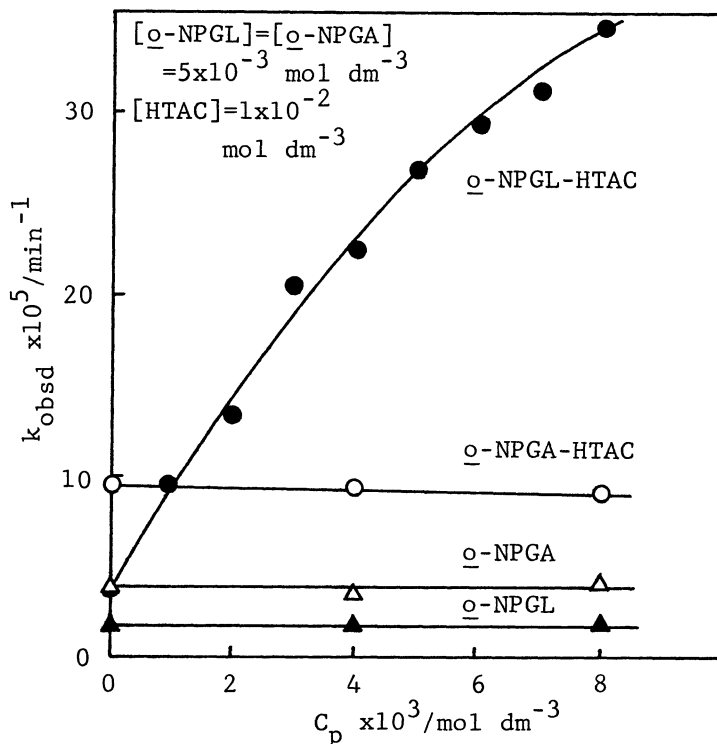
Fig.1. Plots of pseudo-first-order rate constants ( k_{\text{obsd}} ) as a function of phenylboronic acid concentration ( C_p ); pH 11.4 at 25°C.
